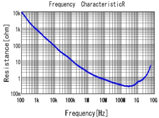
GCM155R71H102KA37 R DCOV, 25degC
