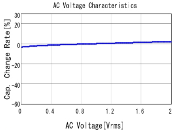
GCM155R71H102KA37 C-AC Voltage capchange, DCOV, 25.0d
