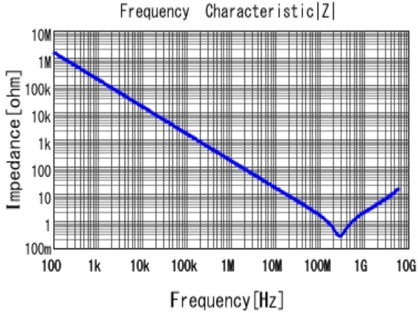
GCM155R71H102KA37 |Z| DCOV, 25degC
