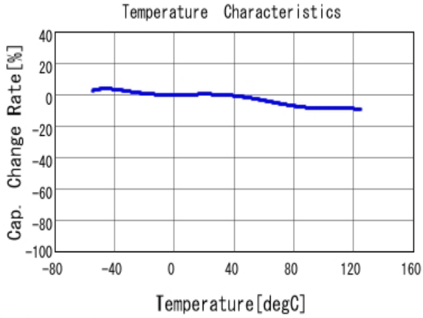
■ GCM155R71H102KA37 C-Temp. capchange, DCO. 0V, AC1.0V rm
