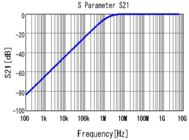
■ GCM155R71H102KA37 S21 DCOV, 25degC
