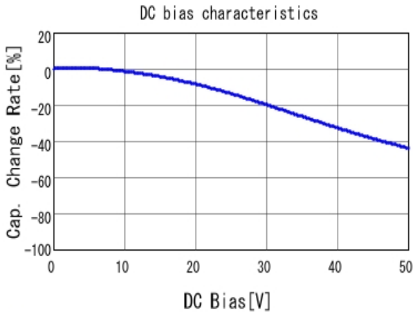
GCM155R71H102KA37 C-DC bias capchange, 25.0degC, AC1.
