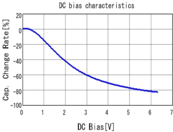
■ GRM188R60J226MEA0 C-DC bias capchange, 25.0degC, AC0.
