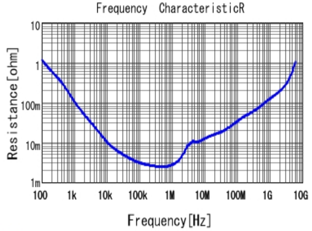
■ GRM188R60J226MEA0 R DCOV, 25degC
