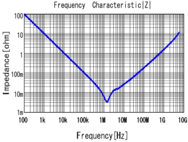
■ GRM188R60J226MEA0 |Z| DCOV, 25degC
