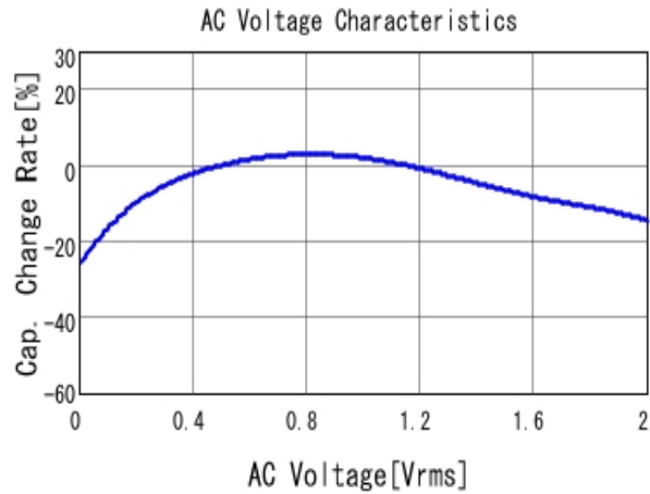
■ GRM188R60J226MEA0 C-AC Voltage capchange, DCOV, 25.0d
