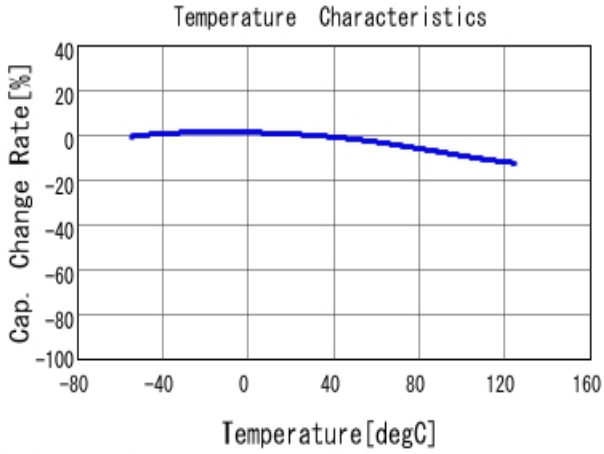
■ GRM32ER71H475KA88 C-Temp. capchange, DC0.0V, AC1.0V rm
