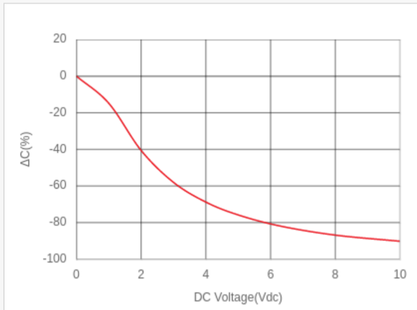
DC Bias Characteristics LCR meter, 1kHz, 0.5Vrms
