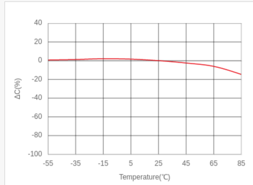
Temperature Characteristics of Capacitance(TCC) LCR meter, 1kHz, 0.5Vrms
