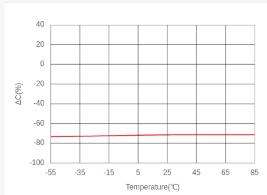
Bias TCC Characteristics LCR meter, 1kHz, 0.5Vrms, 5Vdc
