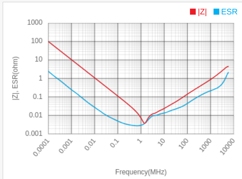
Frequency Characteristics Network Analyzer
