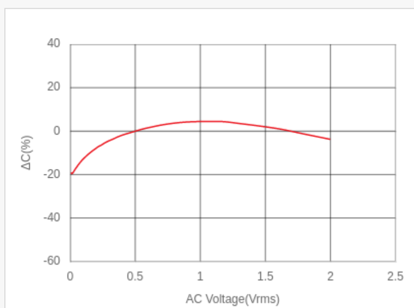
AC Voltage Characteristics LCR meter, 0.12kHz
