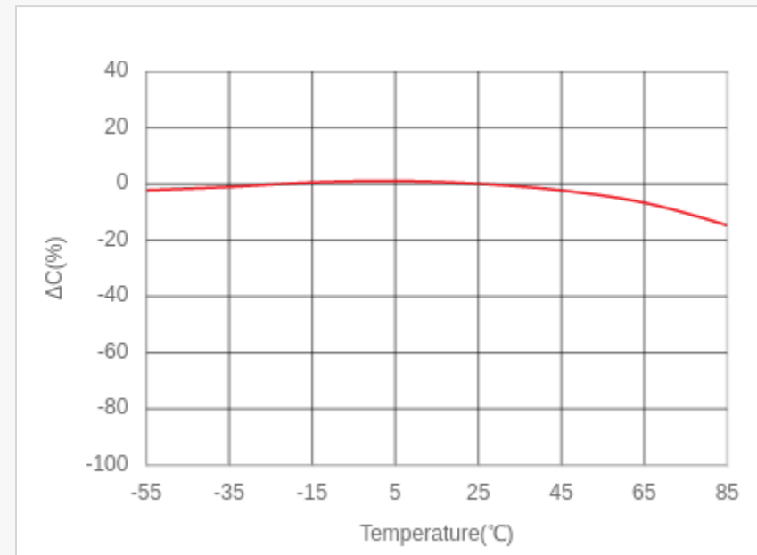
Temperature Characteristics of Capacitance(TCC) LCR meter, 0.12kHz, 0.5Vrms
