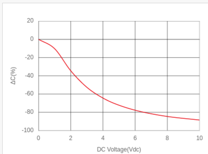
DC Bias Characteristics LCR meter, 0.12kHz, 0.5Vrms
