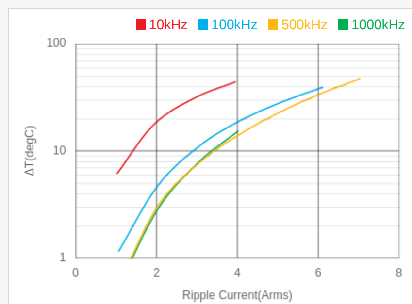
Temperature Rise by Ripple Current
