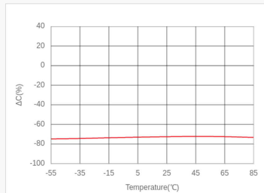
Bias TCC Characteristics LCR meter, 0.12kHz, 0.5Vrms, 5Vdc
