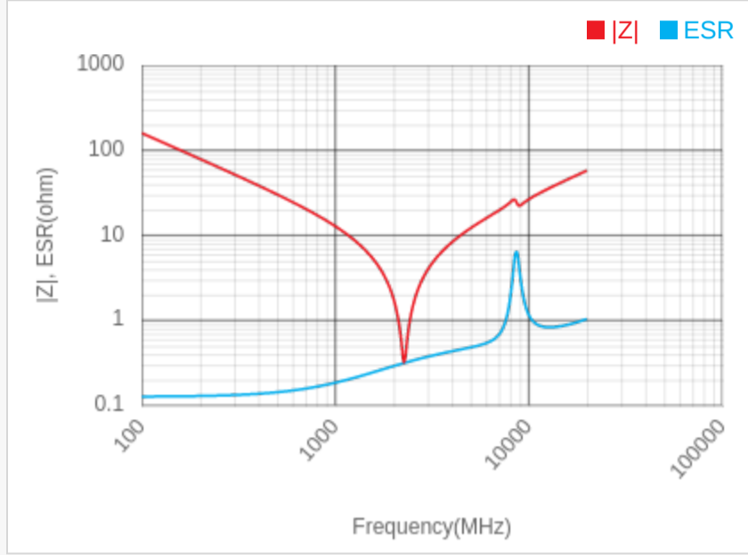
Frequency Characteristics Network Analyzer
