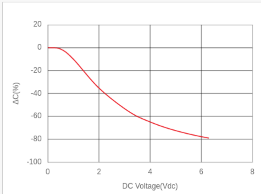
DC Bias Characteristics LCR meter, 0.12kHz, 0.5Vrms
