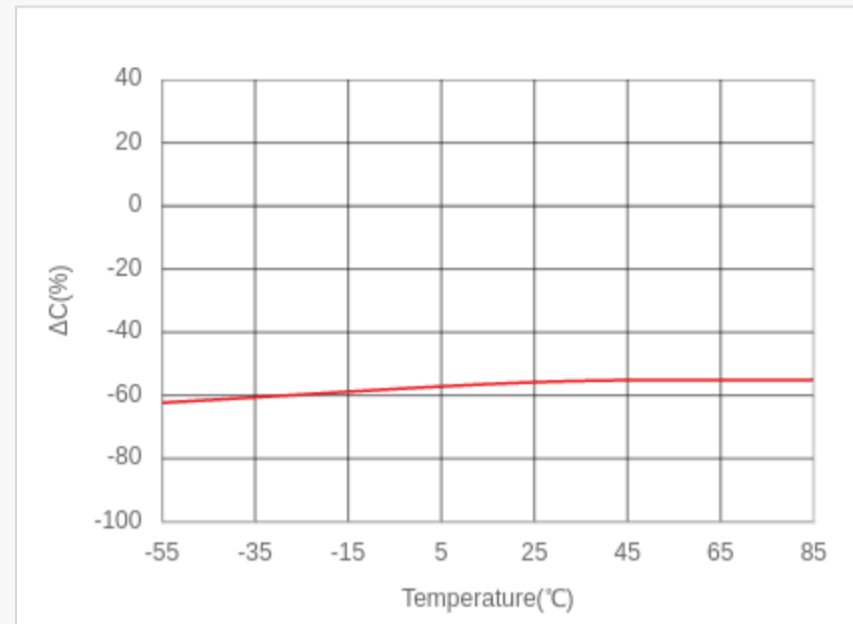
Bias TCC Characteristics LCR meter, 0.12kHz, 0.5Vrms, 3.15Vdc
